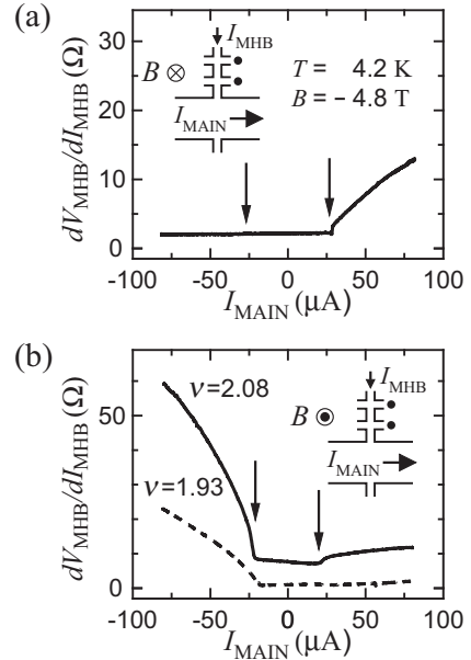
FIG. 4: Differential longitudinal resistance dV_{\text{MHB}}/dI_{\text{MHB}} with I_{\text{MHB}} = 0.2 \mu\text{A} in the upper micro Hall bar. (a) Data at the reversed magnetic field. (b) Data at \nu = 1.93 (dashed curve) with I_{\text{cr}} = 19.9 \mu\text{A} and \nu = 2.08 (solid curve) with I_{\text{cr}} = 21.0 \mu\text{A} (indicated by arrows).
